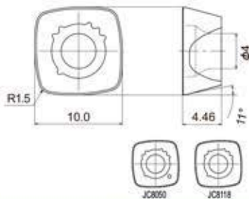
Fig.1 SPNW100415ZTR
