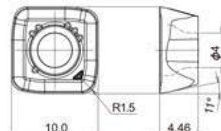
Fig.3 SPMT100415ZPER-SM
